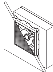
Q 15 M da incasso a muro in-wall, for wall made of bricks
