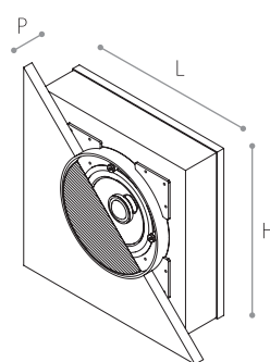
T 17 M da muro, incassata in-wall, for wall made of bricks
